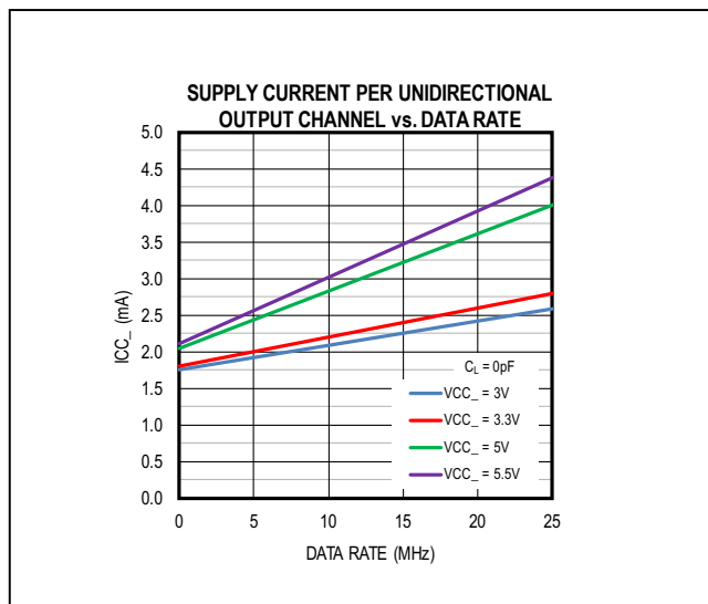
Figure 6. Supply Current per Output Channel (Estimated)
